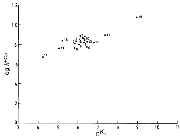
Fig. 10 \log k^{\text{SO}_2} versus \text{p}K_3 plot at 25 °C for \text{cis}(\text{en})_2\text{Co}(\text{B})\text{OH}^{2+} : B = \text{NH}_3 (1), \text{MeNH}_2 (2), \text{EtNH}_2 (3), \text{C}_6\text{H}_5\text{CH}_2\text{NH}_2 (4), \text{C}_6\text{H}_{11}\text{NH}_2 (5), imidazole (6), benzimidazole (7), N -Me-imidazole (8), \text{OH}_2 (9); [(\text{NH}_3)_5\text{CoOH}]^{2+} (10); [(\text{tren})\text{Co}(\text{OH}_2)\text{OH}]^{2+} [tren = tris(2-aminoethyl)amine] (11); [(\text{tetren})\text{CoOH}]^{2+} (12); \beta\text{-cis}[(\text{tren})\text{Co}(\text{OH}_2)\text{OH}]^{2+} (13); [(\text{NH}_3)_5\text{PtOH}]^{3+} (14); [(\text{NH}_3)_5\text{RhOH}]^{2+} (15); [(\text{NH}_3)_5\text{CrOH}]^{2+} (16); \text{trans}[(\text{salen})\text{Cr}(\text{OH}_2)\text{OH}] (17); and \text{trans}[(\text{salen})\text{Co}(\text{OH}_2)\text{OH}] (18).
