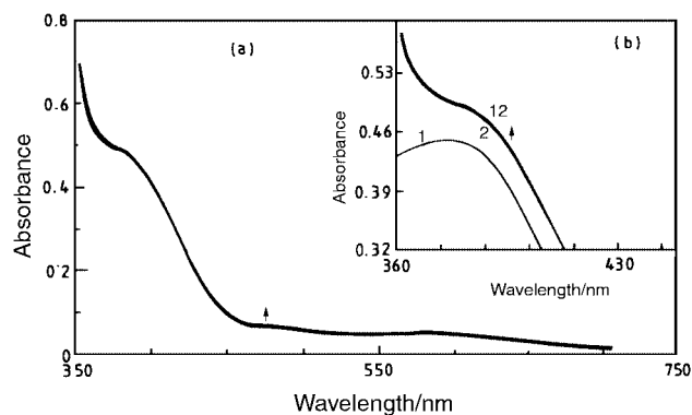
Fig. 4 Rapid scan spectra of \text{trans-[Co(salen)(OH}_2)_2]^+ + \text{S}^{\text{IV}} at 25 °C. [\text{Complex}]_T = 1.0 \times 10^{-4} + [\text{S}^{\text{IV}}]_T = 0.02 \text{ mol dm}^{-3} (pH 6.39, self buffered). (a) number of scans = 96, total time = 0.120 s; (b) inset: curve 1 for complex alone; curves 2–12 for the reaction mixture in 0.12 s; \Delta t = 0.012 \text{ s} between successive runs.
